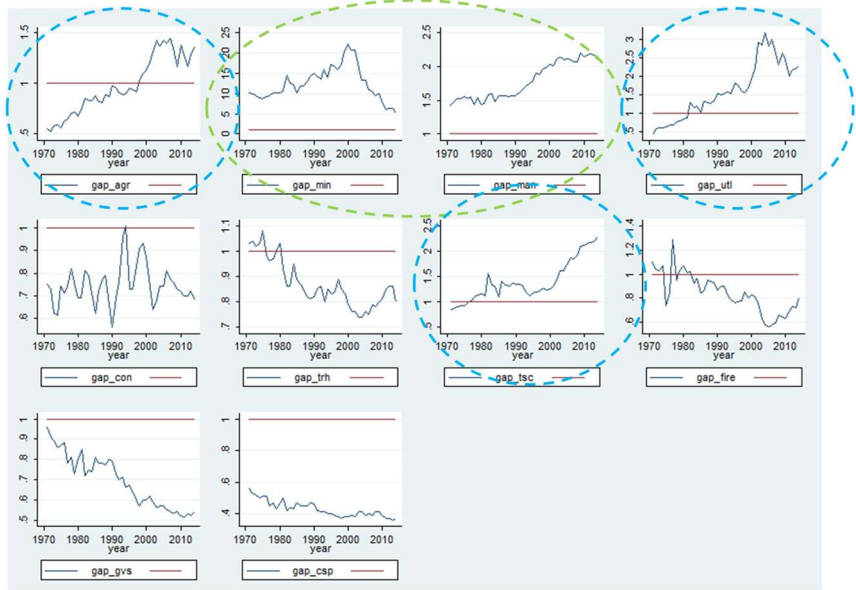
Figure 3.6 Argentina: Evolution of labour productivity gaps by sector (to economy-wide) 1971-2014
